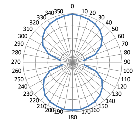
Angular Sensitivity (Relative Read Range vs. Orientation)
